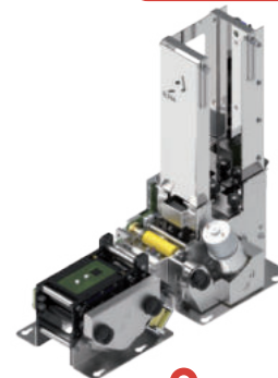
CDU - ELS10000 SERIES Card Dispenser unit w/capture + RFID
