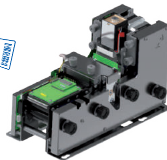
RPTD - ELG9000-RC2 TP SERIES RFID Paper Ticket Dispenser
